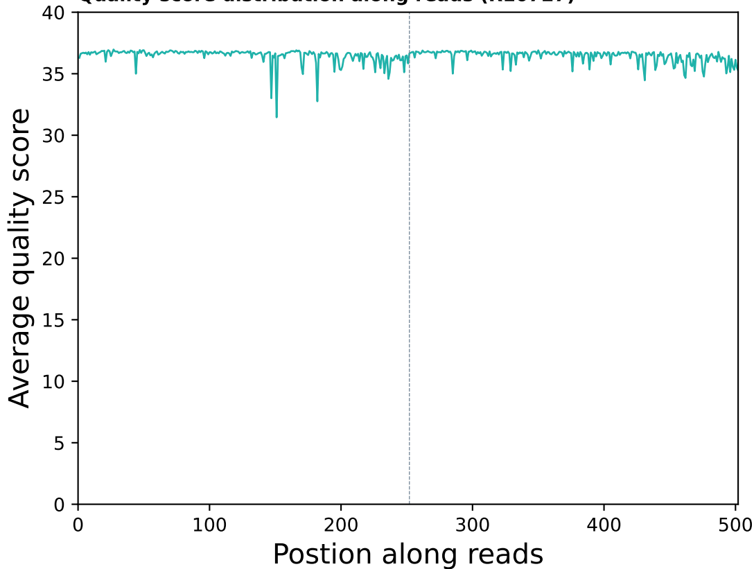
Quality score distribution along reads (R10727)
